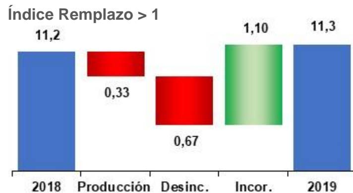
RESERVAS 1P
