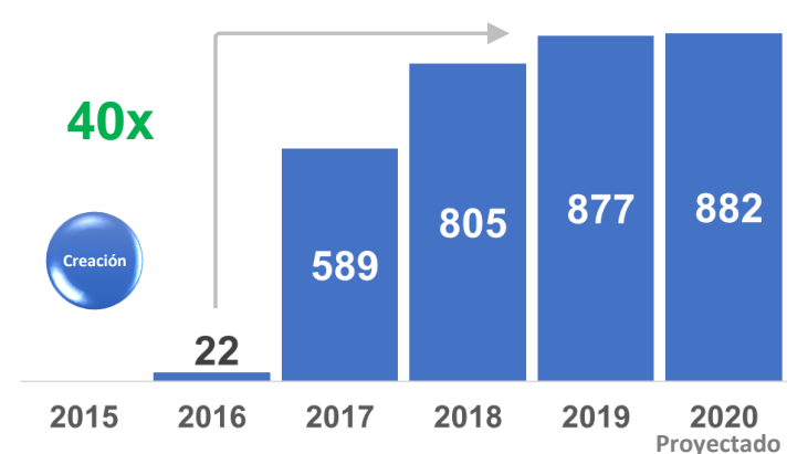
RESERVAS 1P
